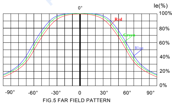
FIG.5 FAR FIELD PATTERN
