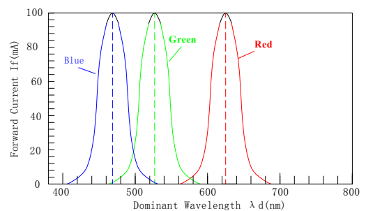
Luminous Spertum ( T_a=25^\circ\text{C} ) SPECTRAL RADIANCE
