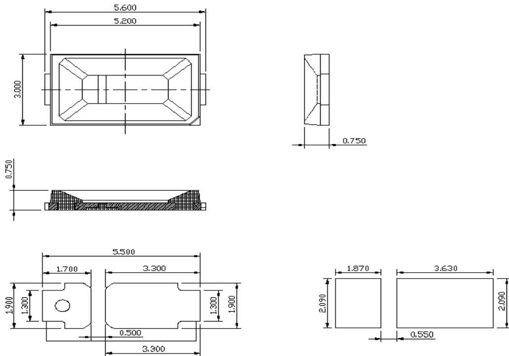
Recommended Solder Pattern
